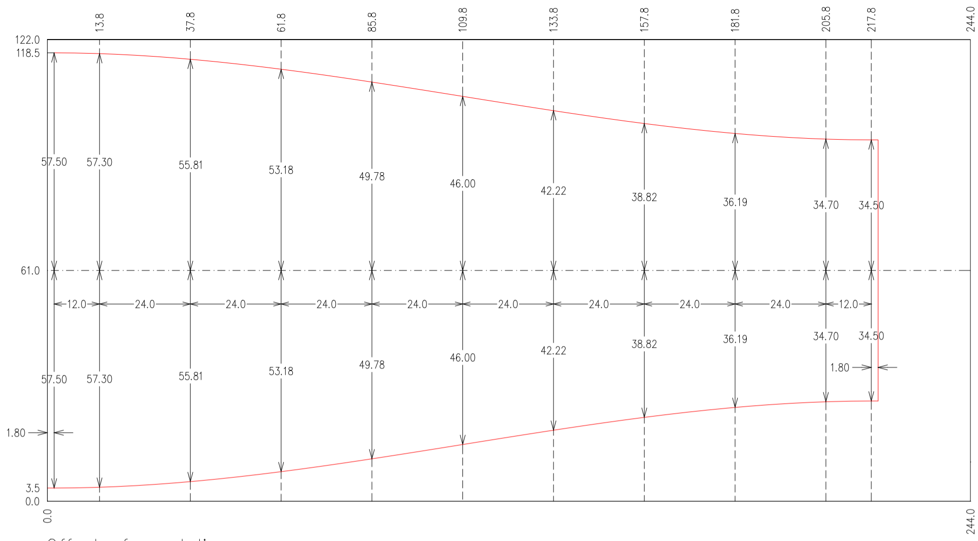
Offsets for cut lines
